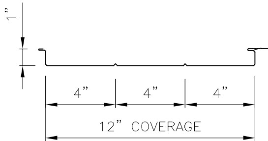
MARQUEE-LOK PROFILE (Double Pencil Rib Optional)
