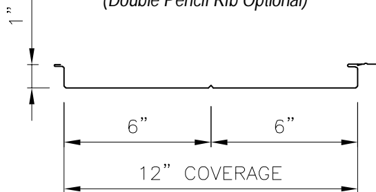
MARQUEE-LOK PROFILE (Single Pencil Rib Optional)
